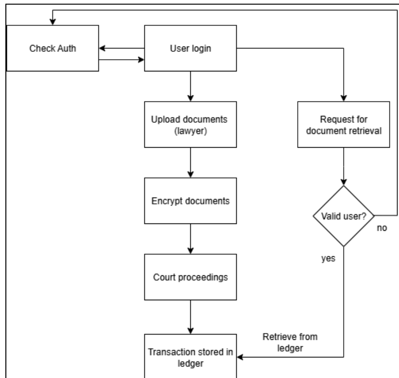
Fig 4.2.4 Flow Diagram
