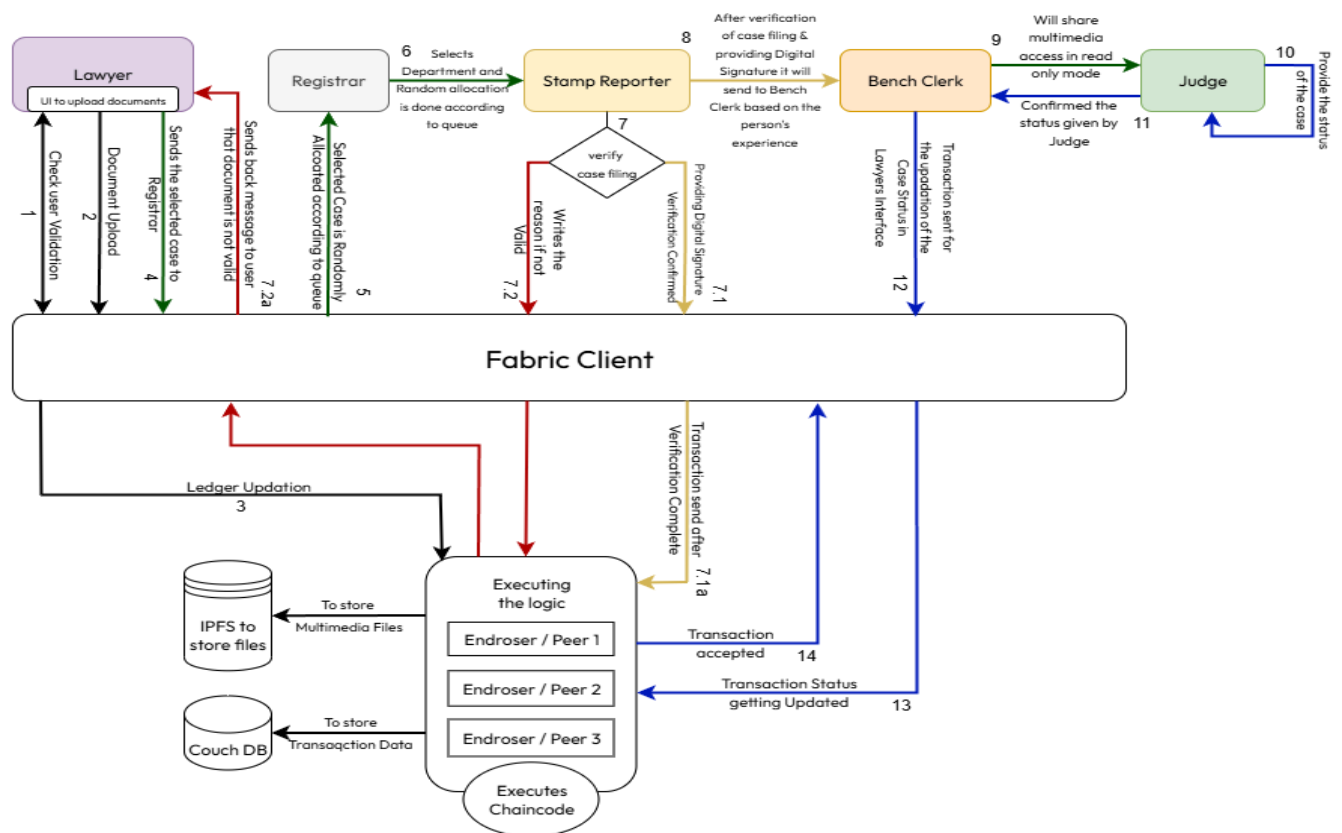
4.1.1 Architecture Diagram
