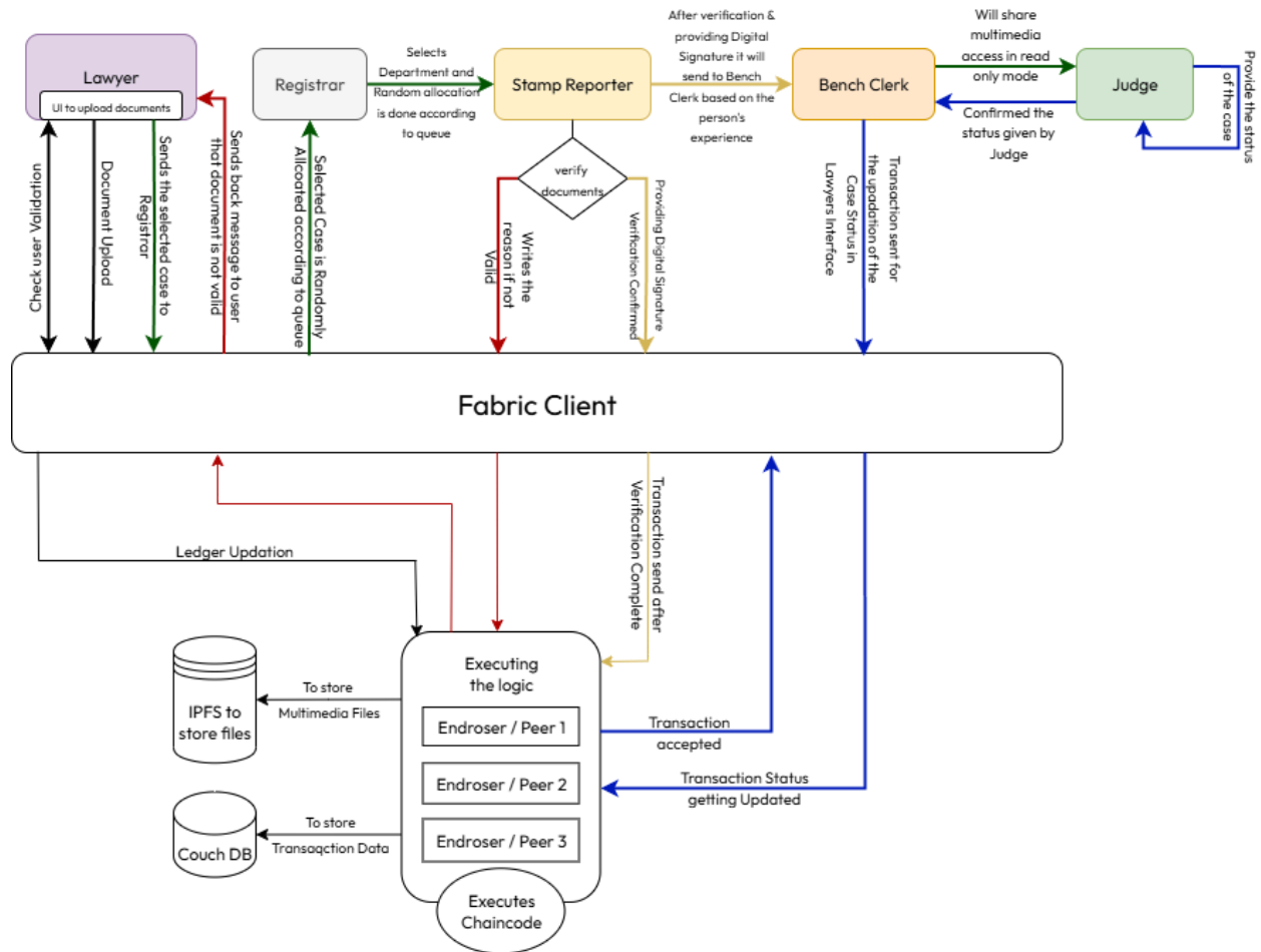
Figure 1 : System architecture diagram of LawLedger
