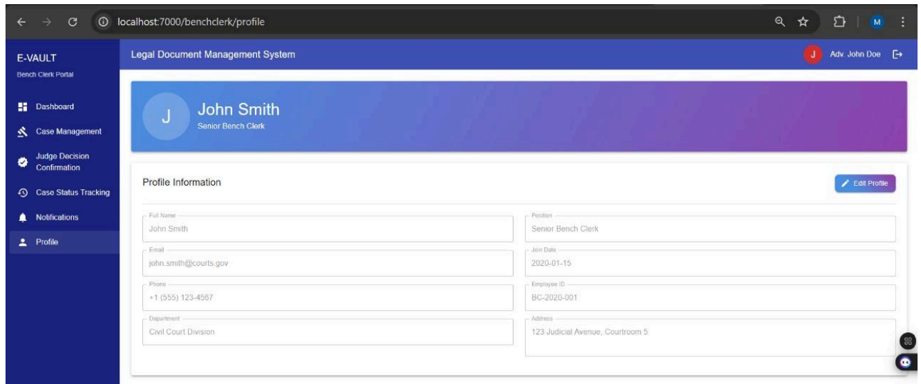
Fig 5.1.1.3 (f) Profile page for the bench clerk
